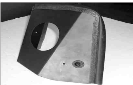
25. Install the rubber grommet that was removed in step 12 and install into heat shield as shown.
