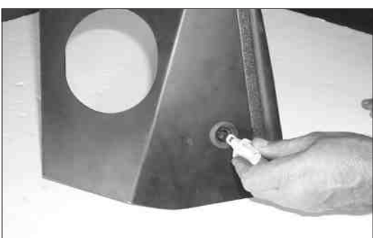
26. Install the air temp sensor that was removed in step 12 into the heat shield as shown.
