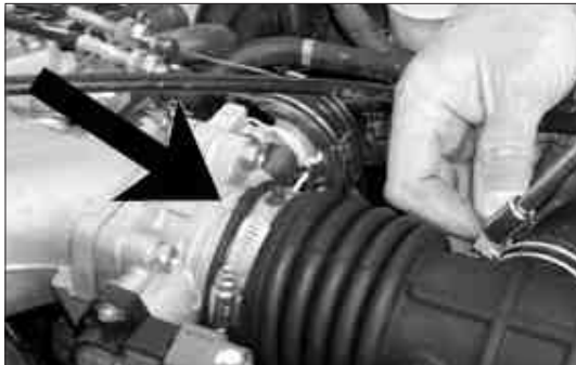
8. Loosen clamp at the throttle body using an 8mm socket.
