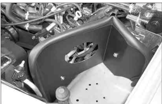
27. Install the heat shield into the vehicle as shown using the provided hardware.
