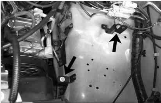
23. Install the two "L" brackets onto the vehicle as shown using the provided hardware. NOTE: Do not tighten completely.
