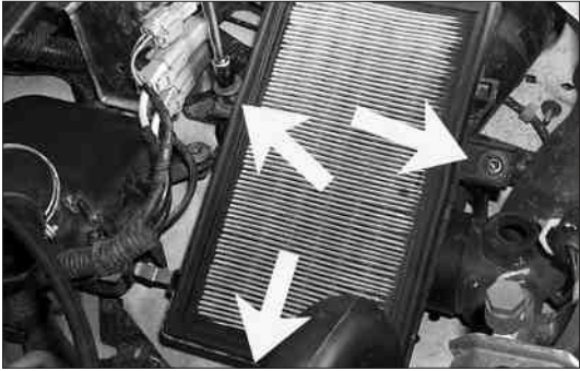
13. Remove the three bolts that secure the lower air filter housing using an 10mm socket.
