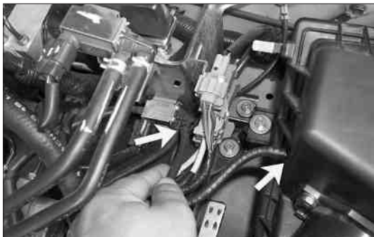
9. Remove vacuum line from bypass solenoid as shown. NOTE: It's the vacuum like that connects to the airbox lid.
