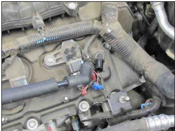
22. Remove the crank case vent tube from the valve cover port.
